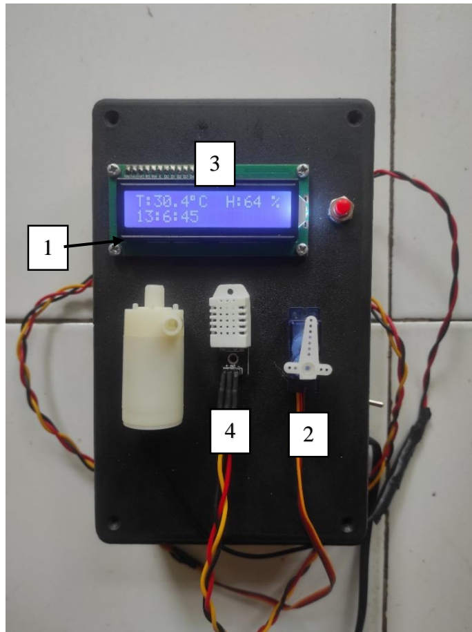
Gambar Hasil Pengujian RTC DS3231 (1), Motor Servo (2), LCD (3), DHT22 (4)
